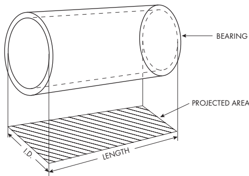
Figure 4: Bearing Pressure
