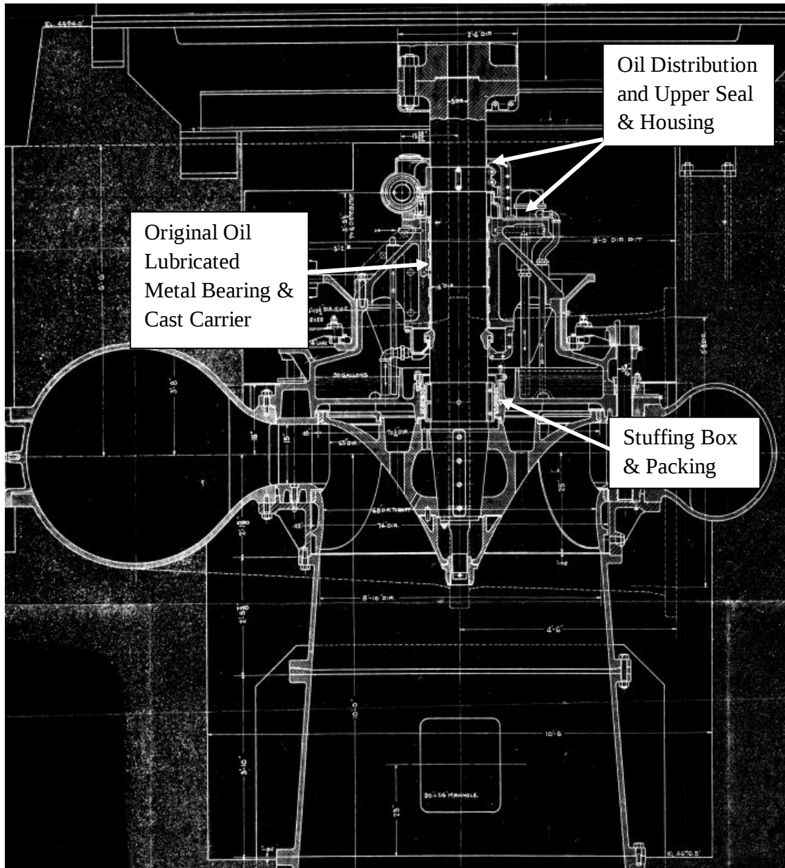
Figure 2: Cross Section of Original Turbine Assembly
