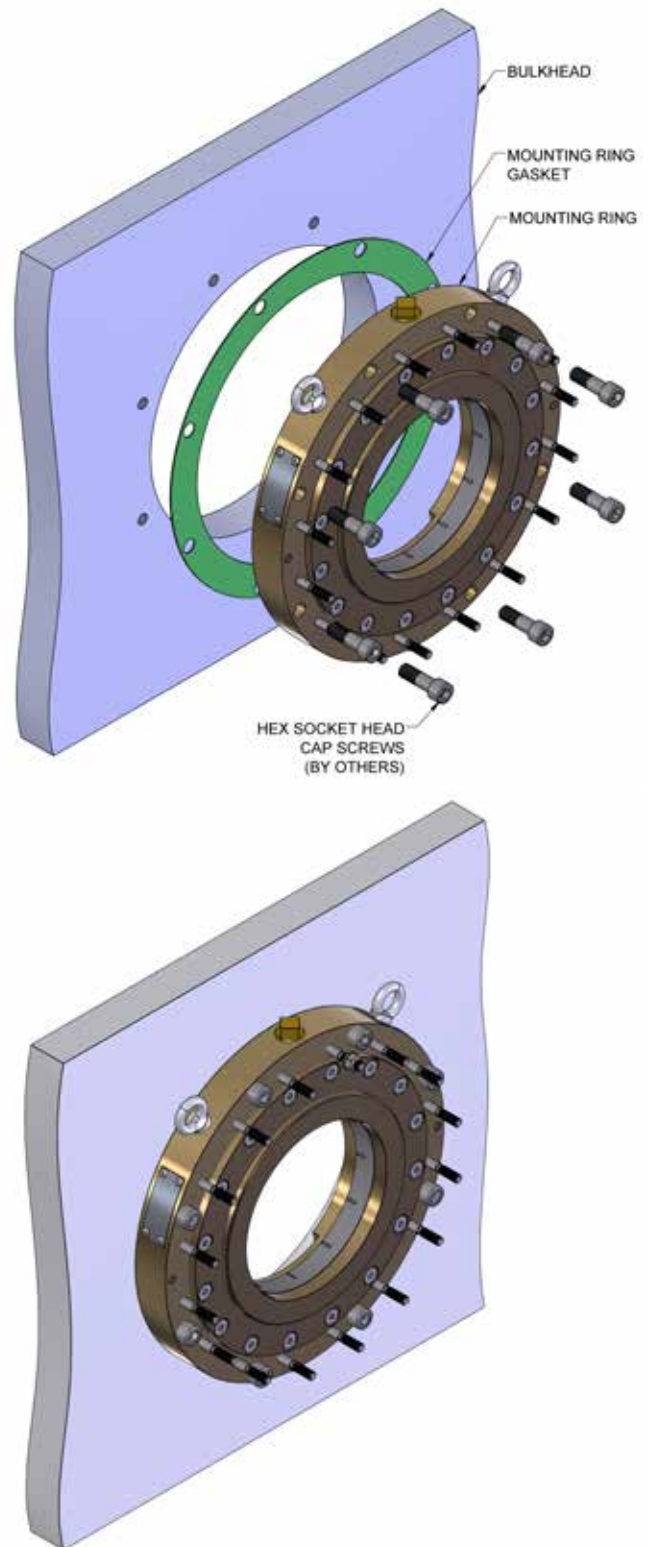
Figure 6: Inflatable Seal and Mounting Ring Fitting
