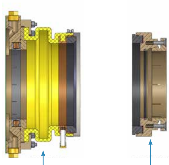
Figure 1: Stationary Seal Subassembly
