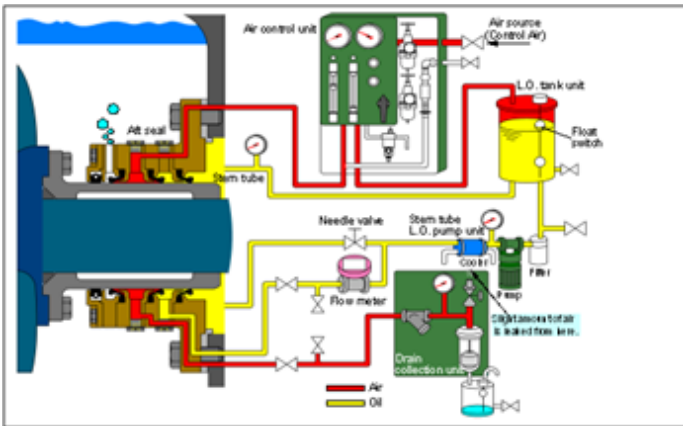
Fig. 2. Oil lubricated system with Typical AFT air seal
