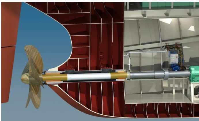
Fig. 4. Typical seawater lubricated propeller shaft bearing system
